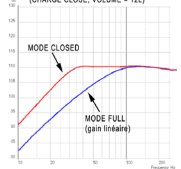
REPONSE EN FREQUENCE DU LD230CR04 (CHARGE CLOSE, VOLUME = 12L)
