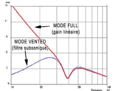
EXCURSIONS DU LD230CR04 (100W) EN CHARGE BASS-REFLEX, VOLUME = 23L, ACCORD 39Hz
